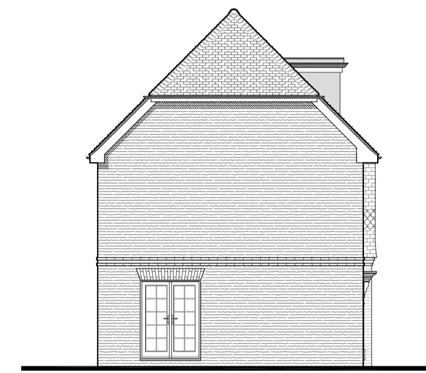
SIDE ELEVATION NORTH-EAST ASPECT - Plot 2 NORTH-EAST ASPECT - Plot 3
